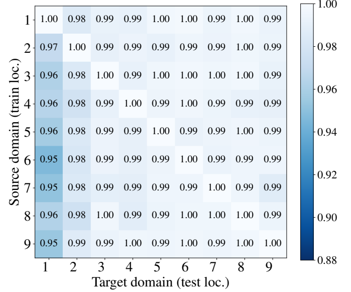
Fig. 12: Pairwise cross-domain transfer accuracy at k = 15 . Each cell represents the accuracy obtained when training on a given source domain and testing on a target domain.
