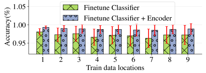
Fig. 15: Cross-domain identification performance of BeamID with and without fine-tuning the encoder.
