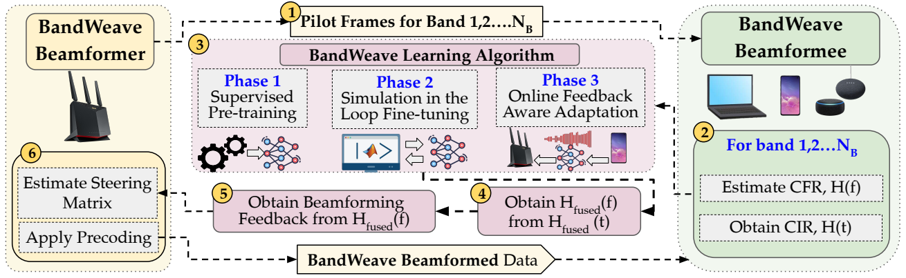
Fig. 5: BANDWEAVE Walkthrough. The numbers in the figure indicate the steps of the processing.
