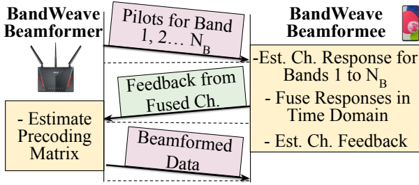
Fig. 2: Overview of BANDWEAVE. ‘Ch.’ stands for channel.
