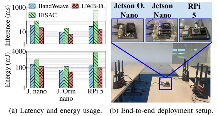
Fig. 14: Inference time and energy consumption of the fusion algorithms implemented on Jetson Nano, Jetson Orin Nano, and Raspberry Pi 5.
