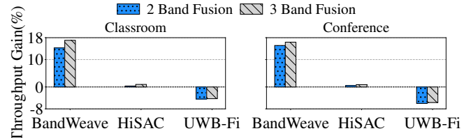
(a) Throughput gain comparison between 2-band (Wi-Fi channel 42 and 58) and 3-band (Wi-Fi channel 42, 58, and 155) fusion.
