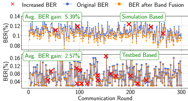
Fig. 4: BER performance evaluation with Algorithm 1.
