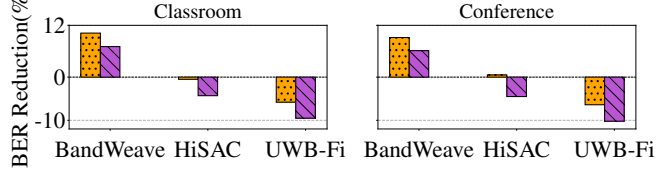
(b) BER reduction with contiguous (centered at 57 & 58 GHz) and non-contiguous bands (centered at 57 & 59 GHz).
