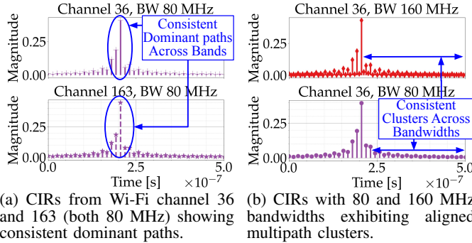
Fig. 3: Multipath analysis through CIR across different center frequencies and bandwidths.
