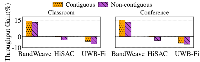
(a) Throughput gain with two 80 MHz bands: contiguous (Wi-Fi channels 42 and 58) and non-contiguous (channels 42 and 155).
