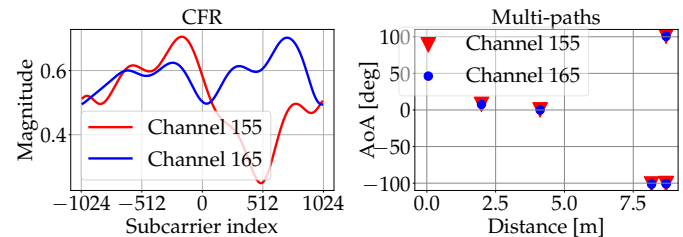
Fig. 1: CFR and multipath decomposition across different Wi-Fi channels (155 and 165).
