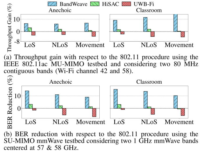
Fig. 8: Communications performance using BANDWEAVE, HiSAC, and UWB-Fi under varying environments and channel conditions. The fused CFR is used for transmission in each of the considered bands and the average performance is reported.
