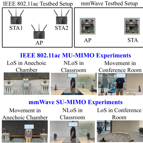
Fig. 7: Experimental scenarios in the anechoic chamber, classroom, and conference room, using both the IEEE 802.11ac MU-MIMO and the mmWave SU-MIMO testbeds.
