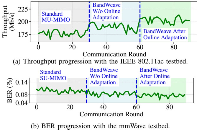
Fig. 12: Impact of BANDWEAVE online adaptation on throughput and BER across communication rounds in conference room with human movement.
