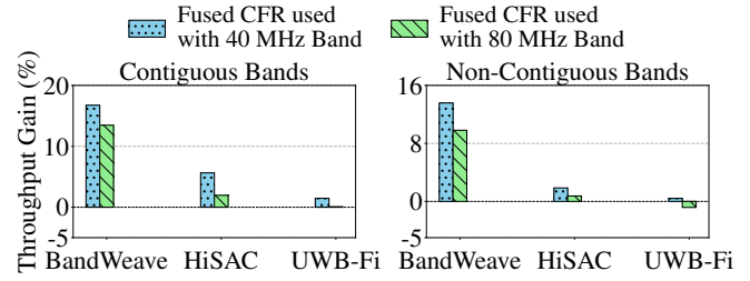
Fig. 10: Throughput gain fusing bands with heterogeneous bandwidths (40 MHz and 80 MHz). Wi-Fi channels 42 and 58 form the contiguous band pair, while channels 42 and 155 are used for the non-contiguous bands.
