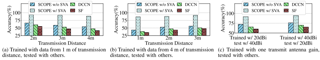
Fig. 4. Performance comparison of SCOPE in generalizing across transmission distances and transmit antenna gains.
