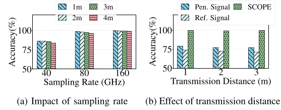
Fig. 3. SCOPE performance illustrating (a) impact of sampling rates on accuracy at different transmission distances and (b) effect of transmission distances on accuracy for penetrating ('Pen.'), reflected ('Ref.'), and combined ('SCOPE') signals.
