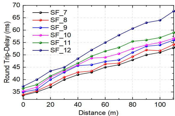
Figure 6. Latency analysis for 500 kHz
