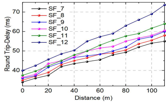
Figure 5. Latency analysis for 125 kHz
