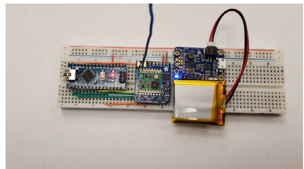
Figure 3. Experimental setup
