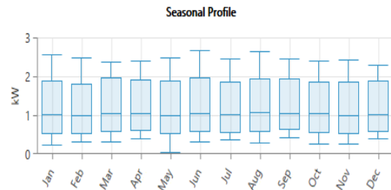
Fig. 4. Monthly load profile
